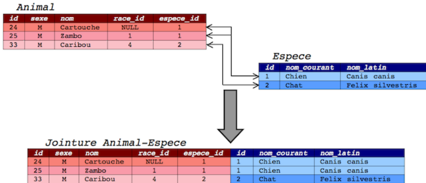
FIGURE 13.1 – Principe des jointures
